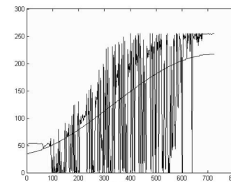
Fitted polynomial line degree 3
