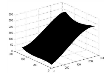
Fitted polynomial surface degree 3
