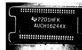
Fig. 7 Binary image
